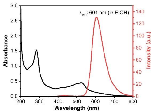
UV/Vis spectra of sulfur doped cyan blue carbon quantum dots
