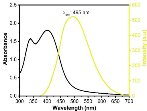
UV/Vis spectra of sulfur doped Yellow carbon quantum dots
